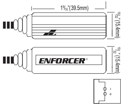
FIG. 6: Dimensions.
