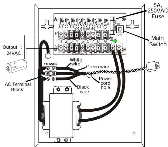
(EVP-1SA4P9UL shown)
