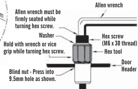
FIG. 6: Mounting the blind nuts in a hollow door or gate post
