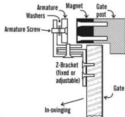
FIG. 5 - Basic Installation
