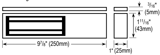
Electromagnet
