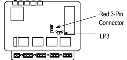
SK-910RAQ/RA-4Q PCB
