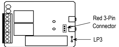
SK-910R3Q/R4Q/R3-4Q/R4-4Q PCB
