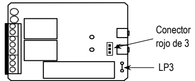
SK-910R3Q/R4Q/R3-4Q/R4-4Q PCB
