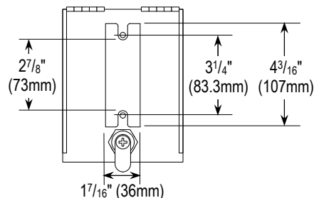
BP-611 Cutout size, shown from inside as opened
