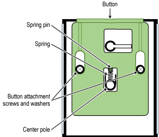
Housing cover – inside view
